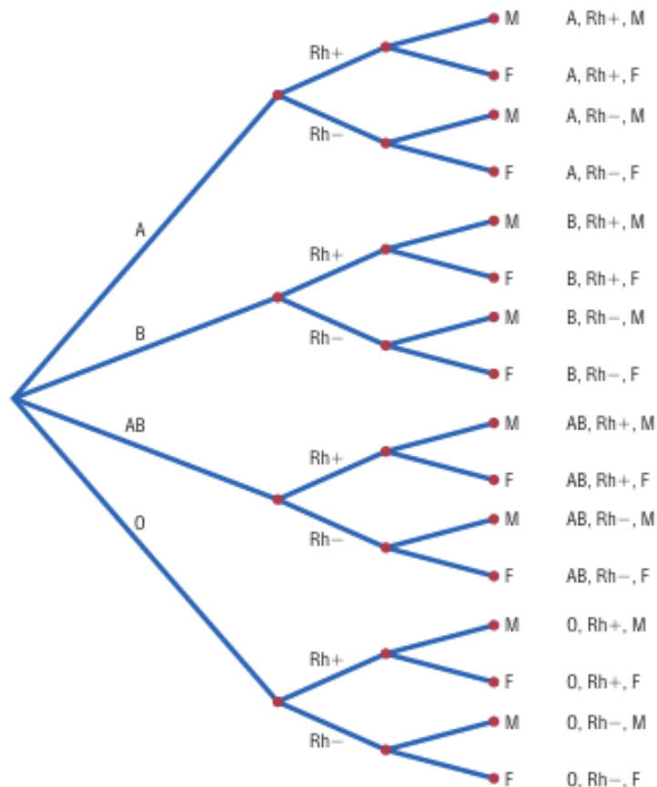
FIGURE 4-11 Complete Tree Diagram for Example 4-40
